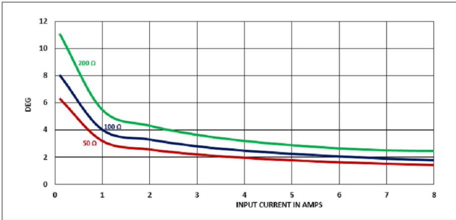
PHASE ANGLE RESPONSE vs INPUT CURRENT @ RATED BURDEN:
