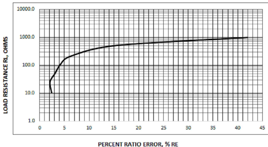
%RE VS RL AT RATED PRIMARY CURRENT @ 7.5A/50HZ
