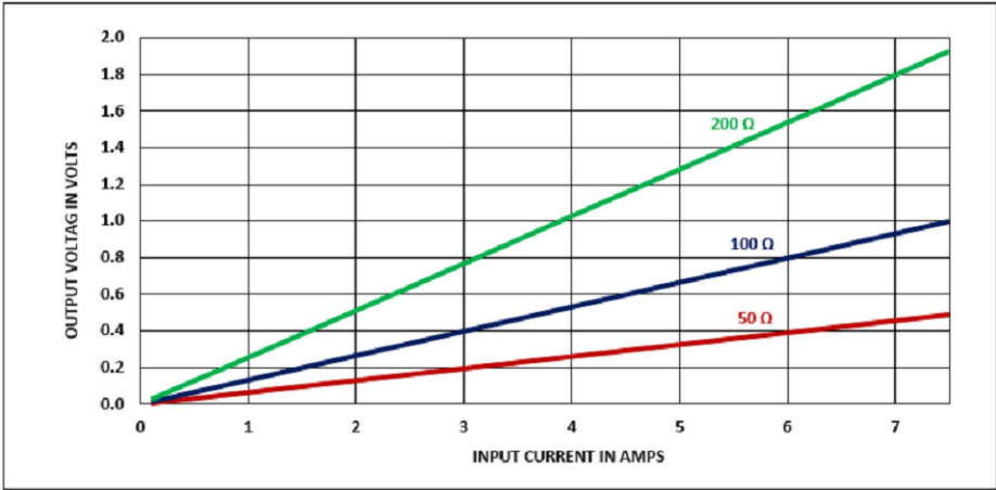
SATURATION CURRENT RESPONSE @ RATED BURDEN:
