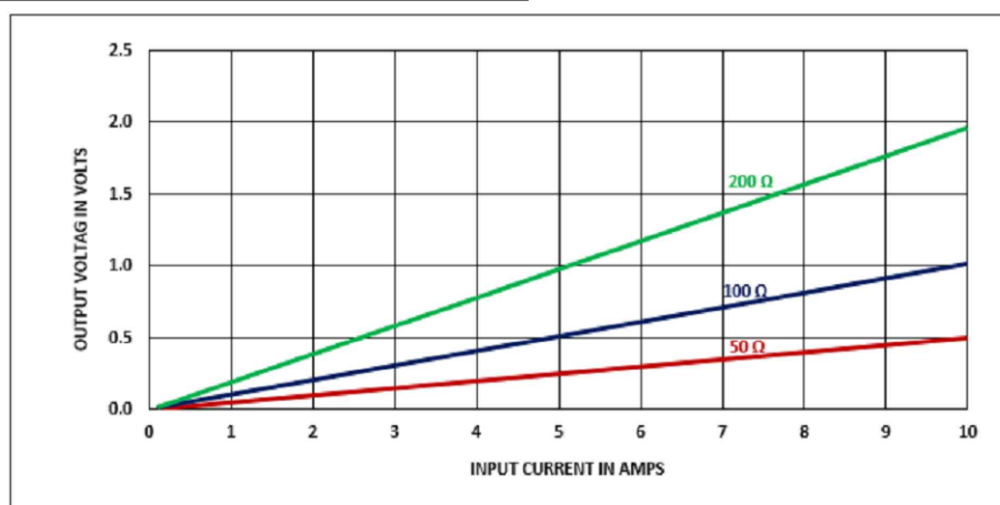
SATURATION CURRENT RESPONSE @ RATED BURDEN:
